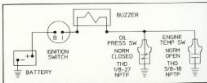
Continually monitors engine oil pressure and engine coolant temperature.
